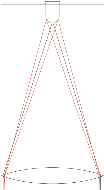
Large Long Focal Length Lens
